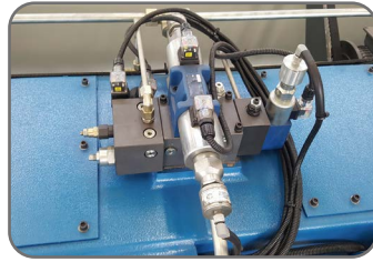
Germany Bosch-Rexroth Hydraulic System
